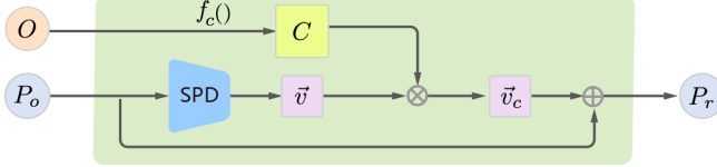
Fig. 5. The structure of offset constrained refinement unit (OCRU). We use function f_c to compute the value C , which is used to constrain the range of movement \vec{v}_c computed by SPD.
