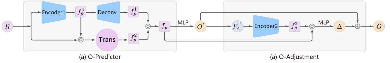
Fig. 4. The structure of the offset prediction module. It contains the initial offset prediction (O-Predictor) and the offset adjustment (O-Adjustment).
