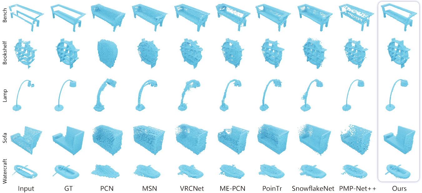
Fig. 7. Visualized completion results for comparison on MVP dataset.
