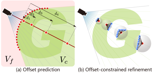
Fig. 2. The completion along rays. (a) we duplicate the observed point multiple times to get the larger red points, and move them along the ray with offset d_i . (b) we split each red point multiple times to get the blue points and spread them to a neighborhood of the red point (the transparent circle).
