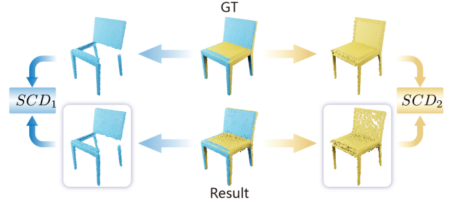
Fig. 6. The computation of SCD_1 and SCD_2 .
