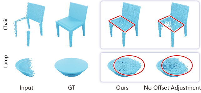
Fig. 8. Ablation study: compare our method with the version that has no offset adjustment step.
