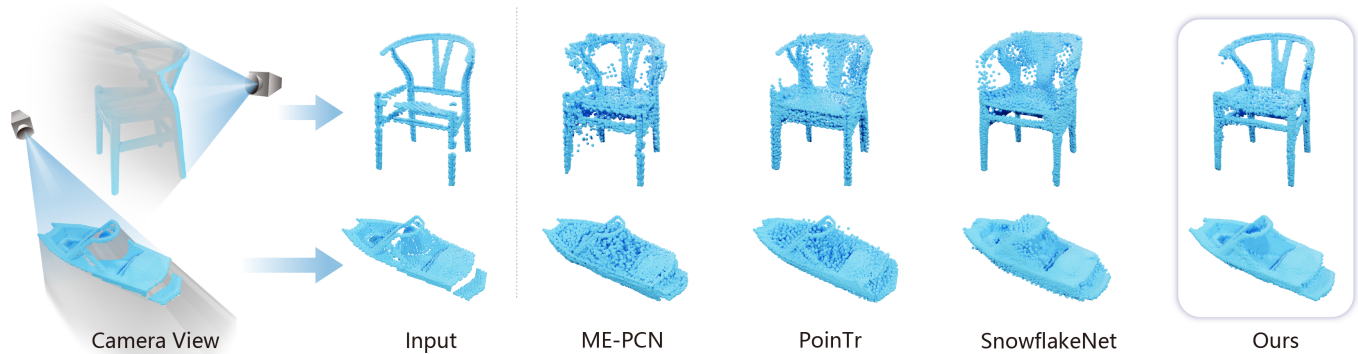
Fig. 1. Given a single-view partial scan, our method considers the volume that is shadowed by the observed points and generates more complete and clean results compared with ME-PCN [Gong et al. 2021], PoinTr [Yu et al. 2021] and SnowflakeNet [Xiang et al. 2021].
